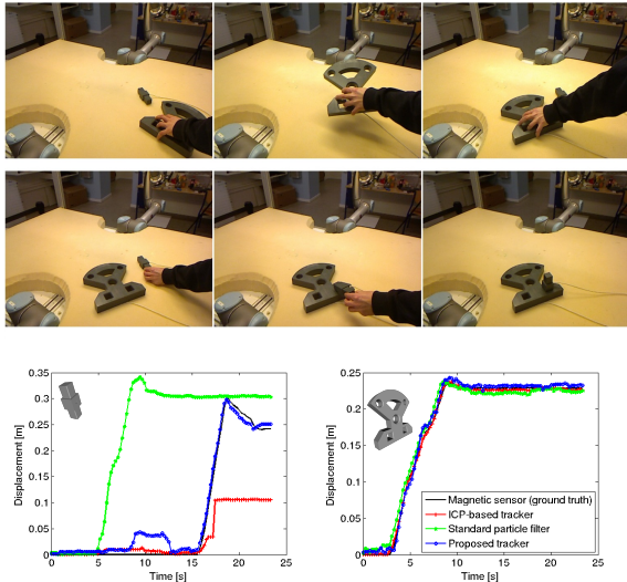
Figure 8: Results for a peg in hole assembly sequence. See text for details.
