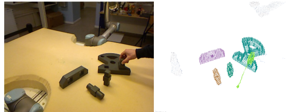
Figure 1: Left: intermediate frame of a complex assembly scene where one of many peg in hole operations is being performed. Right: detection and tracking output.
