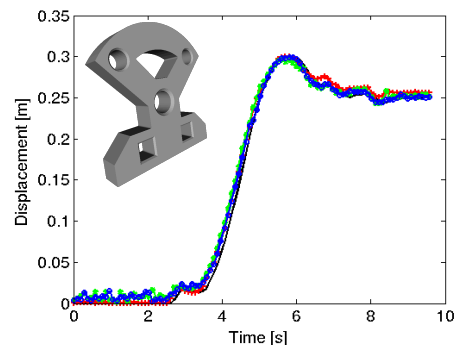
Figure 7: Results for the simple sequences. The object is moved along a circular arc during manipulation.
