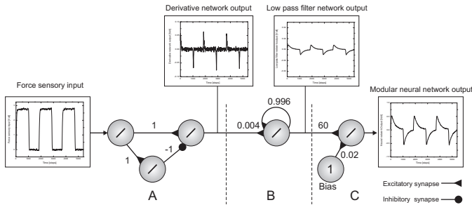
Fig. 4. Modular neural network with a linear activation function of all neurons. It consists of three modules: (A), (B), and (C). All synaptic weights indicated by the small numbers were manually tuned.
