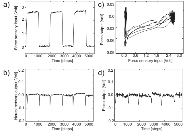
Fig. 5. a) Force sensory input from the FSR at the sole during simulated walking driven by the setup shown in Fig. 2c. It is used as an input of the neural model of the piezoelectric energy harvesting system. b) The output of the neural model which was trained to obtain a desired response of the piezoceramic MFC. c) Nonlinear relation between the force sensory input and the response of the piezoceramic MFC. d) The response of the piezoceramic MFC during simulated walking. All filtered signals are recorded at a sampling rate of 10 kHz.
