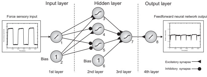
Fig. 3. Feedforward neural network with linear activation functions for input and output neurons and symmetric sigmoid activation functions (i.e., tanh) for hidden neurons. The weights ( \omega from neuron j to neuron i ) were trained by a backpropagation algorithm. The resulting weights are \omega_{31} = 0.142 , \omega_{32} = 0.062 , \omega_{41} = -0.679 , \omega_{42} = 0.221 , \omega_{51} = -1.012 , \omega_{52} = -0.493 , \omega_{73} = 0.049 , \omega_{74} = -0.360 , \omega_{75} = 0.422 , \omega_{76} = 0.143 , \omega_{87} = 4.0 .
