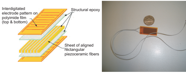
Fig. 1. (a) Schematic of a piezoceramic MFC structure [7]. (b) Piezoceramic MFC arrays.
