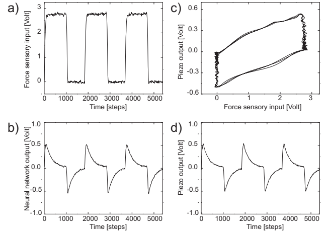
Fig. 6. a) Force sensory input from the FSR at the heel during simulated walking. It is used as an input of the neural model of the piezoelectric energy harvesting system. b) The output of the neural model which shows a similar pattern to the response of the piezoceramic MFC. c) Nonlinear relation between the force sensory input and the response of the piezoceramic MFC. d) The response of the piezoceramic MFC during simulated walking. All filtered signals are recorded at a sampling rate of 10 kHz.
