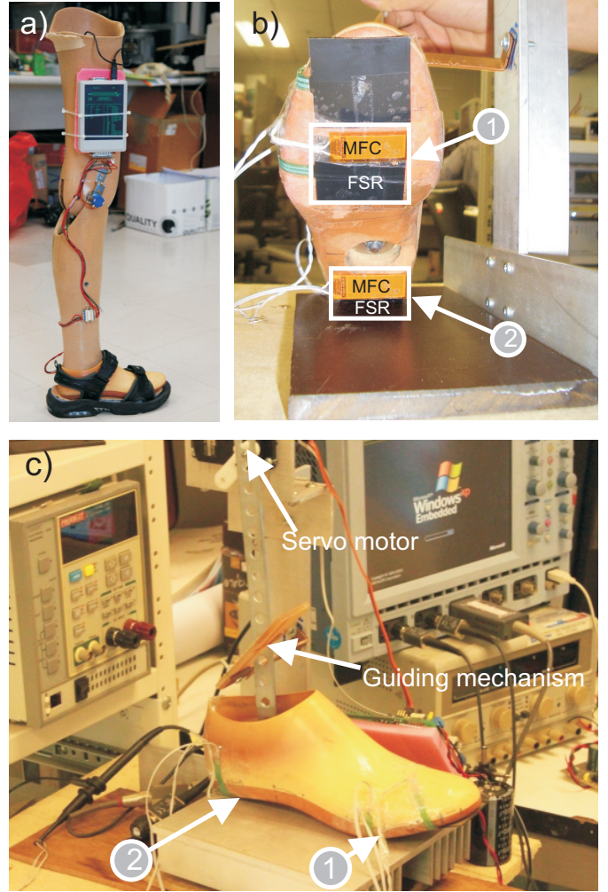
Fig. 2. (a) Prosthetic leg donated by Rehabilitation Research Institute (RRI). It is modified by installing the sensors and the piezoelectric materials to be used as an experimental platform. (b) Installation of the piezoceramic MFCs and the force sensing resistors (FSRs) at the sole (1) and heel (2) of the leg. (c) Experimental setup to simulate walking behavior and to record the force sensory signals and the electrical power generated by the piezoceramic MFCs.
