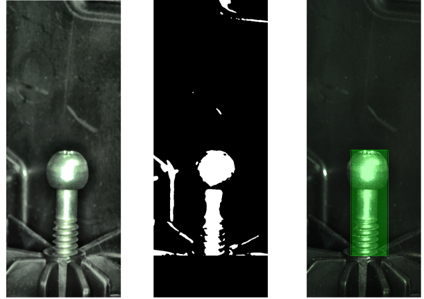
Figure 10: The screw is detected using connected component analysis.
