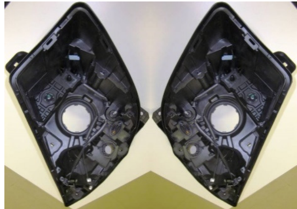
Figure 2: Two models of left and right automotive light housings produced by Elvez. Left: Housing X07; Right: Housing X82.
